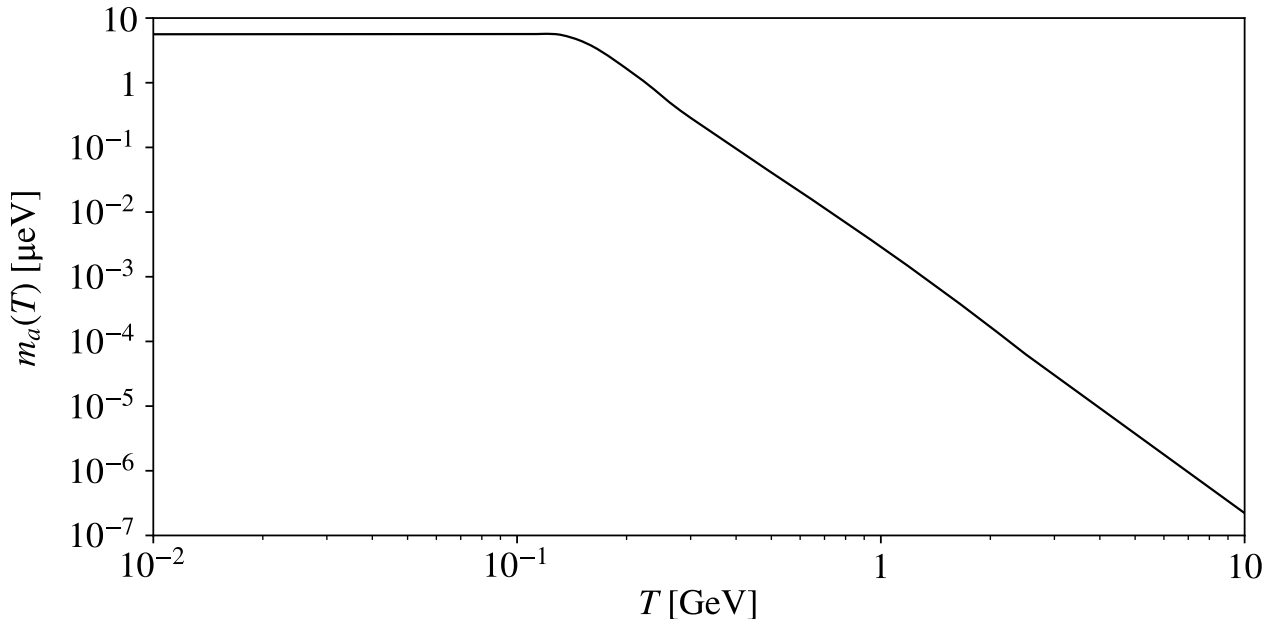
Figure 1: The mass of the axion as a function of the temperature for f_a = 10^{12} GeV, using the data provided in ref. [25].
